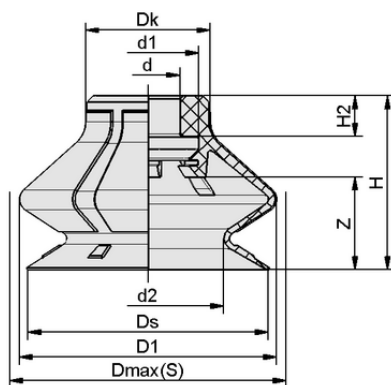
Design data SPB1 60 ED-65 SC050
