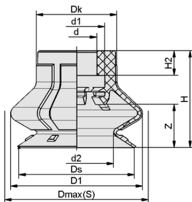
Design data SPB1 30 ED-65 SC040
