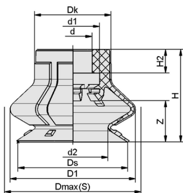
Design data SPB1 20 ED-65 SC040
