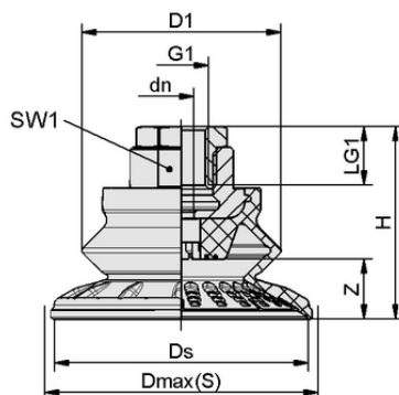
Design data SAB 22 HT2-65 G3/8-IG
