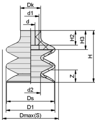
Design data FG 52 NK-45 N018
