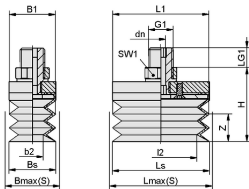
Design data FSGB-R 60x29 NBR-50 G1/4-AG
