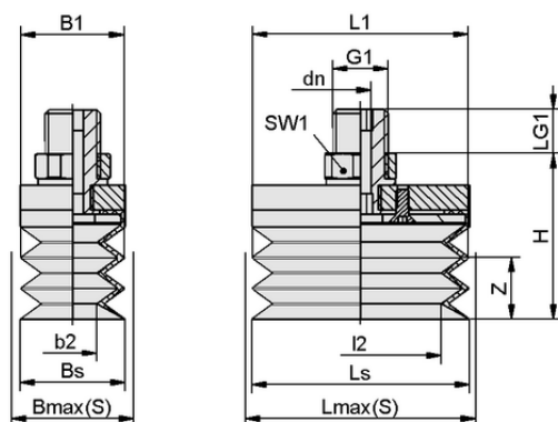
Design data FSGB-R 52x25 SI-50 G1/4-AG
