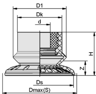
Design data SABT 80 NBR-60
