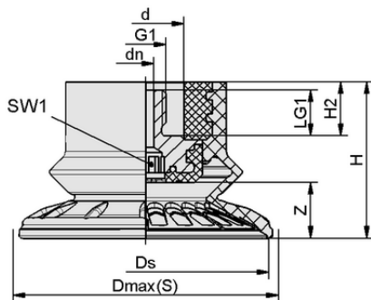
Design data SABT-C 60 NBR-60 M10-AG
