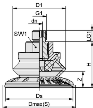
Design data SAB 22 NBR-60 G1/4-AG
