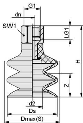
Design data FSG 32 HT1-60 G1/4-IG
