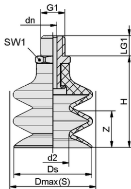
Design data FSG 5 HT1-60 M5-AG
