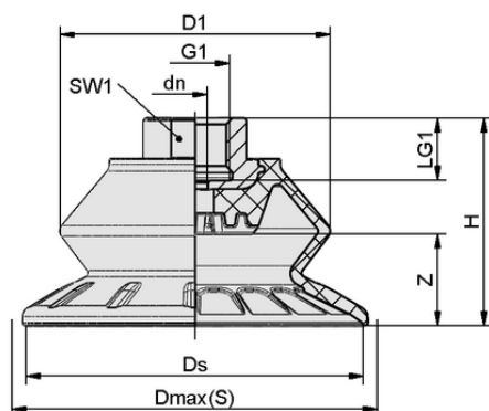
Design data SAB 30 NBR-60 G1/4-IG
