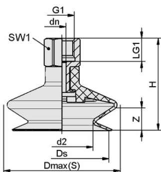
Design data FSGA 25 HT1-60 G1/8-IG
