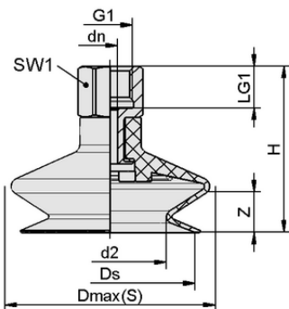
Design data FSGA 20 HT1-60 G1/8-IG
