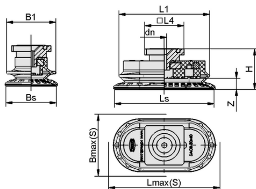
Design data SAOB 60x30 NBR-60 RA
