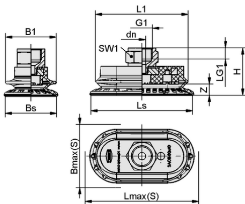
Design data SAOB 80x40 NBR-60 G3/8-IG
