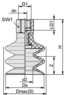
Design data FSG 5 NBR-55 M5-IG
