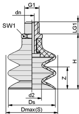
Design data FSG 52 NBR-55 G1/4-AG
