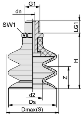
Design data FSG 12 NBR-55 M5-AG
