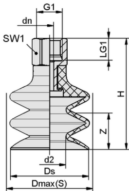
Design data FSG 18 NK-45 G1/8-IG
