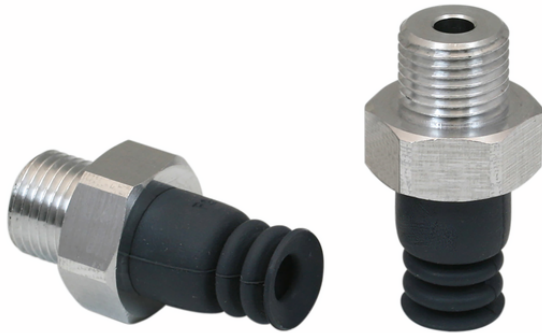
FSG 9 NK-45 G1/8-AG
