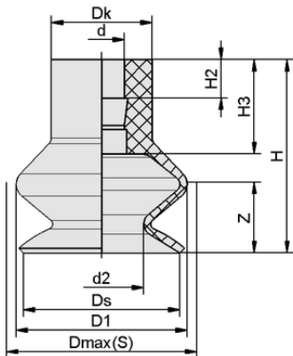
Design data FGA 14 NBR-55 N016
