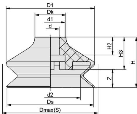
Design data FGA 40 VU1-72 N011 ON
