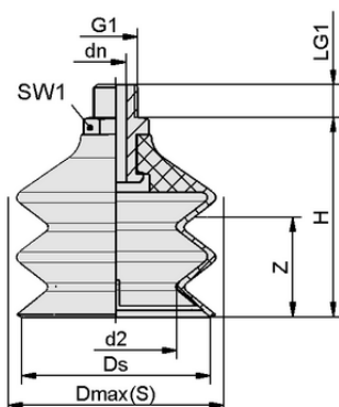
Design data FSG 85 VU1-72 G1/4-AG ON
