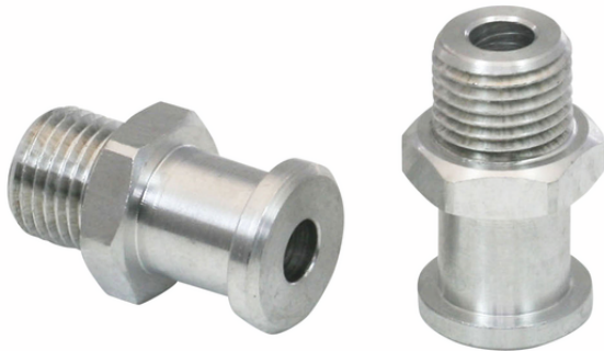
SA-NIP N014 G1/4-AG DN600
