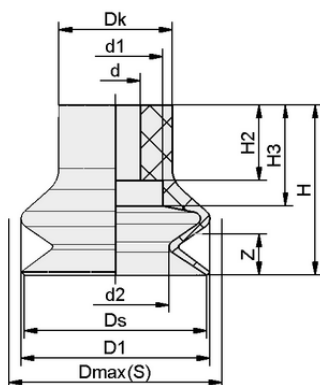
Design data FGA 30 VU1-72 N013
