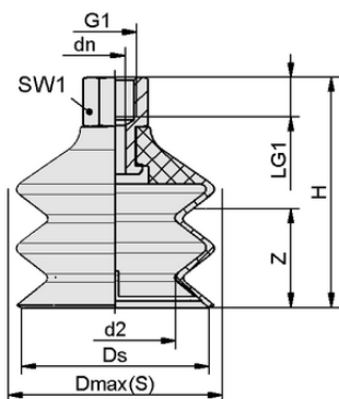
Design data FSG 60 VU1-72 G1/4-IG ON
