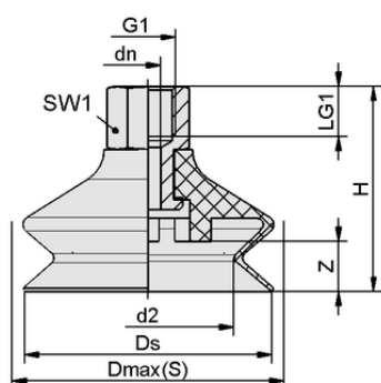
Design data FSGA 30 VU1-72 G1/4-IG
