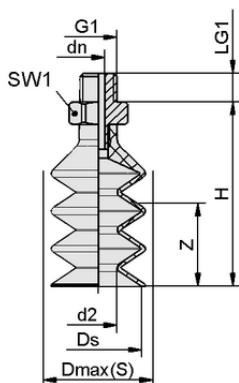
Design data FSGB 25 NBR-55 G1/8-AG
