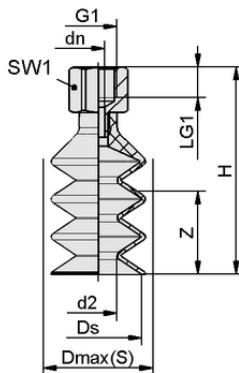
Design data FSGB 25 SI-55 G1/8-IG
