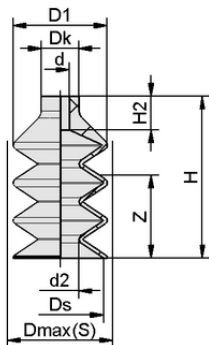
Design data FGB 25 NBR-55 N049
