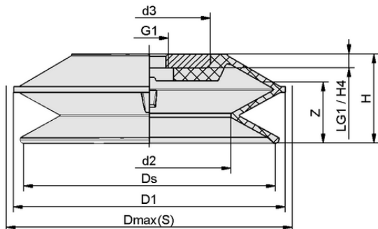
Design data FSGPL 250 NBR-55 G1/2-IG
