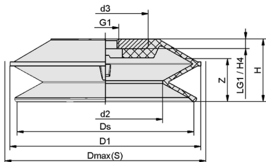
Design data FSGPL 150 NBR-55 G1/2-IG
