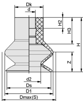
Design data FGA 11 SI-55 N016
