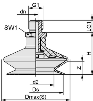
Design data FSGA 78 SI-55 G1/4-AG
