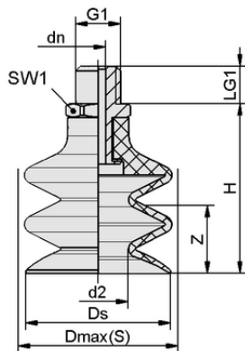
Design data FSG 14 SI-55 M5-AG
