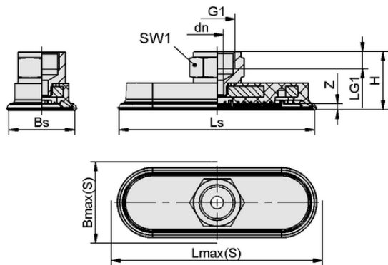
Design data SAOF 140x70 NBR-45 NPT3/8-IG
