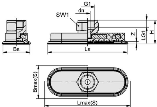
Design data SAOF 80x40 HT2-65 G3/8-IG
