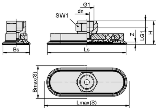
Design data SAOF 50x16 NBR-45 G3/8-IG
