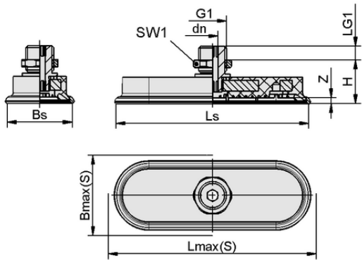
Design data SAOF 50x16 NBR-45 G1/4-AG
