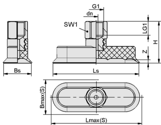
Design data SGON 18x6 HT1-60 M5-IG
