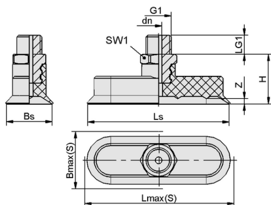
Design data SGON 30x10 HT1-60 G1/8-AG
