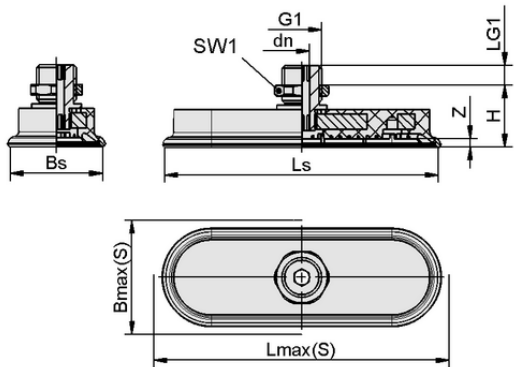
Design data SAOF 60x23 NBR-60 M14x1.5-AG
