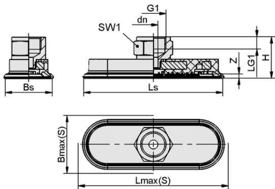
Design data SAOF 60x23 NBR-60 G1/4-IG
