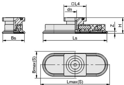
Design data SAOF 90x30 NBR-60 RA
