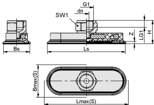
Design data SAOF 80x40 NBR-60 G1/4-IG
