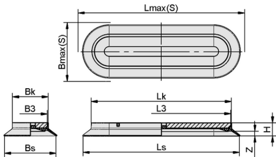
Design data SPLO 250x55 NBR-55
