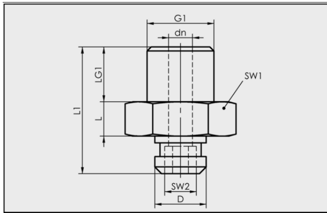
Design data SA-NIP N021 M5-AG DN200
