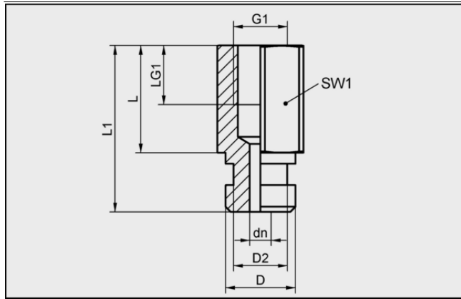
Design data SA-NIP N021 M5-IG DN200
